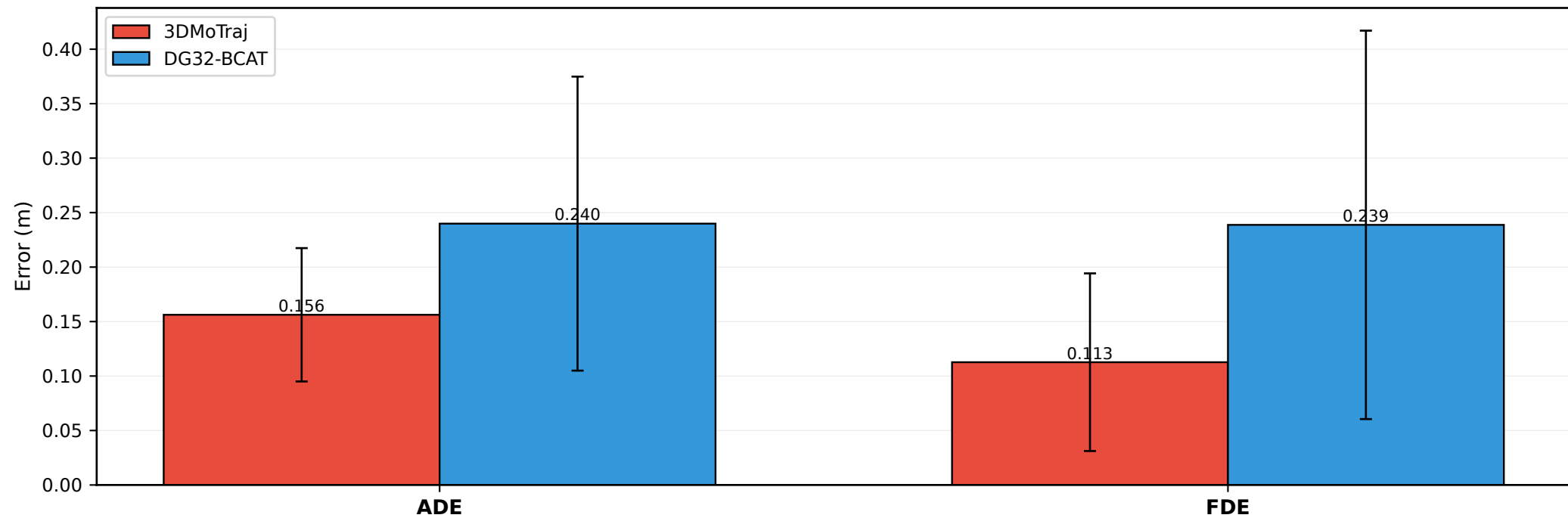
ADE/FDE Comparison: 3DMoTraj vs DG32-BCAT
